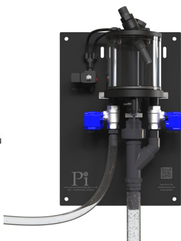
Autoflush Cell PN: 36500001
