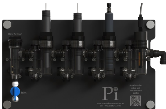
Primary Modular Flow Cells with 3 Additional Cells PN: 32100021
